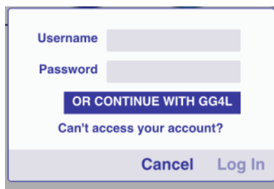
Researcher Login
